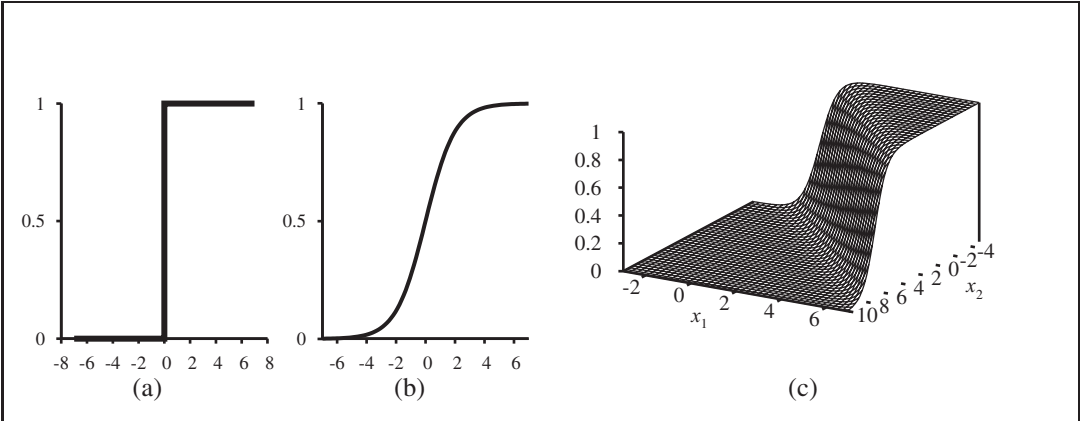
Figure 18.17 (a) The hard threshold function \text{Threshold}(\cdot) with 0/1 output. Note that the function is nondifferentiable at =0 . (b) The logistic function, \text{Logistic}(\cdot) = \frac{1}{1+e^{-z}} , also known as the sigmoid function. (c) Plot of a logistic regression hypothesis h_{\mathbf{w}}(\mathbf{x}) = \text{Logistic}(\mathbf{w} \cdot \mathbf{x}) for the data shown in Figure 18.15(b).
