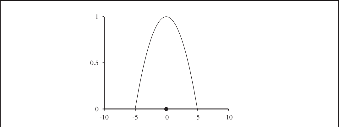
Figure 18.29 A quadratic kernel, \mathcal{K}(x) = \max(0, 1 - (2|x|)^2) , with kernel width = 10 , centered on the query point = 0 .
