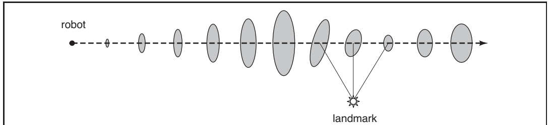
Figure 25.12 Example of localization using the extended Kalman filter. The robot moves on a straight line. As it progresses, its uncertainty increases gradually, as illustrated by the error ellipses. When it observes a landmark with known position, the uncertainty is reduced.
