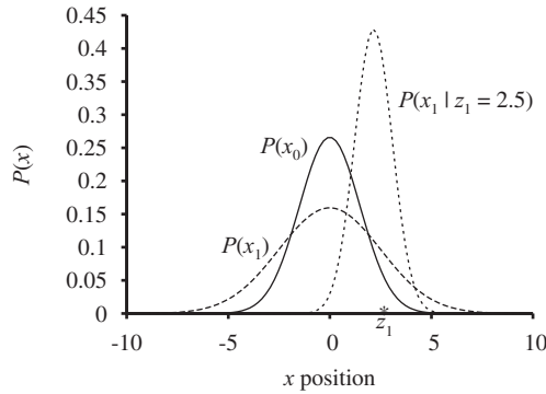
Figure 15.10 Stages in the Kalman filter update cycle for a random walk with a prior given by \mu_0 = 0 and \sigma_0^2 = 1 , transition noise given by \sigma_x^2 = 2 , sensor noise given by \sigma_z^2 = 1 , and a first observation z_1 = 2.5 (marked on the x -axis). Notice how the prediction P(x_1) is flattened out, relative to P(x_0) , by the transition noise. Notice also that the mean of the posterior distribution P(x_1 | z_1) is slightly to the left of the observation z_1 because the mean is a weighted average of the prediction and the observation.
